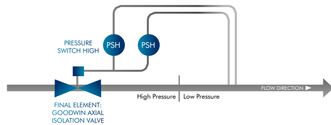
Mechanical HIPPS System (SIL3:1oo2)
