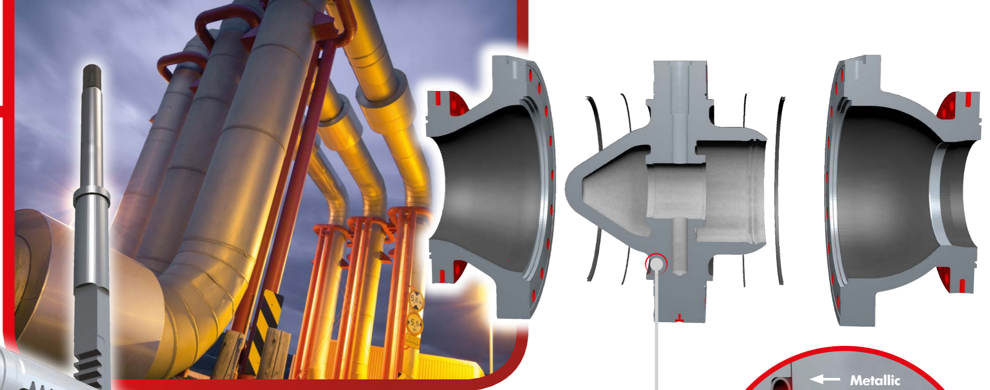
3 PIECE SPLIT BODY DESIGN
