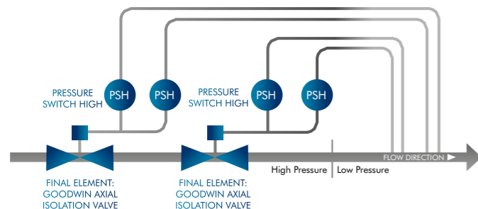
Mechanical HIPPS System (SIL3:1oo2)
