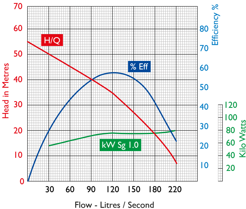
200 HNZZ 112kW, 1450 RPM (50Hz)
